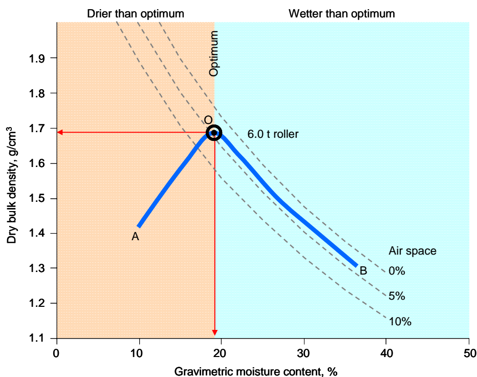
Figure 2 A Proctor compaction curve (blue line) for a cricket loam (loams with clay contents between 26 and 32% all plotted on the same line). Maximum density is 1.68 \text{ g/cm}^3 and this occurs at the optimum moisture content of 19% (black marker and red lines).
